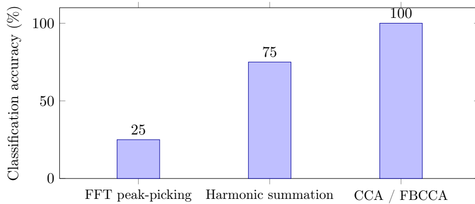
Figure 5: SSVEP single-key classification accuracy by decoding method, single-subject prototype data set ( N = 1 , 5 trials per key). Reconstructed from the accuracy values reported in SSVEP_cVEP_Analysis. Verify exact percentages against the notebook’s current output before final submission. The upward trend (naive FFT → harmonic-aware → correlation-based) matches the pattern predicted by the literature reviewed in Section 2.2.
