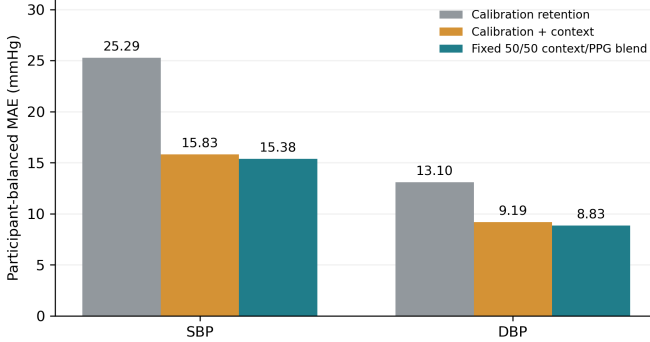
Fig. 2. VitalDB locked-holdout participant-balanced MAE. Calibration-plus-context explains most of the gain over retention; the frozen fixed context/PPG blend adds small CI-supported incremental improvements for both endpoints.
