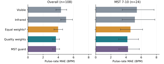
Fig. 1. Participant-balanced pulse-rate MAE with marginal 95% bootstrap intervals. The equal-weight comparison was added post hoc; quality weighting improves overall error relative to equal weighting, while guarded MST correction does not establish additional benefit.
