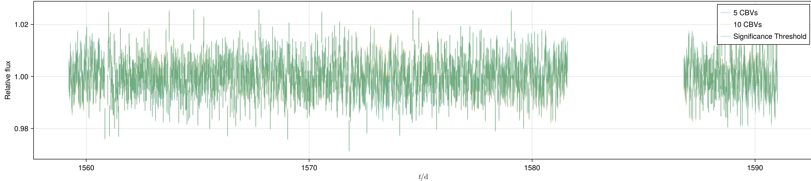
hlsp_iris_kepler_kepler_kplr005025075-q17_kepler_v1.0_lc_detrended.fits
