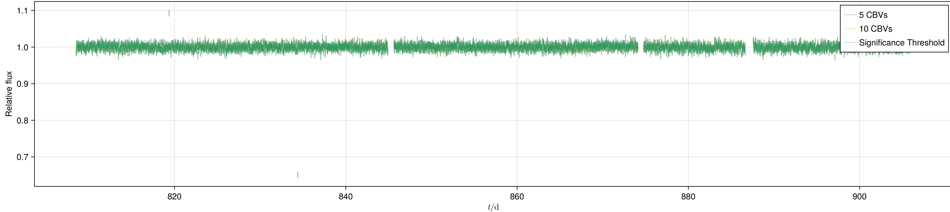
hlsp_iris_kepler_kepler_kplr002438442-q09_kepler_v1.0_lc_detrended.fits
