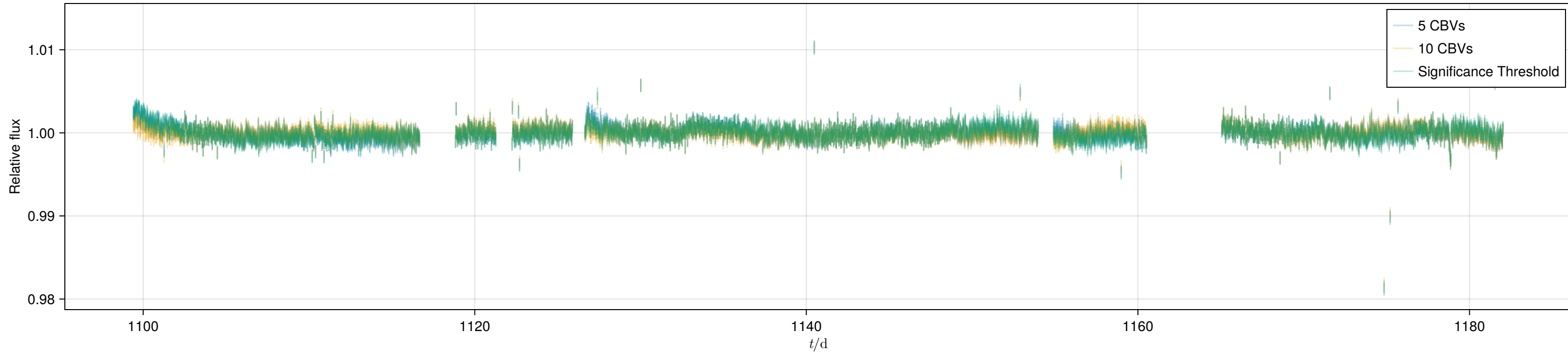
hlsp_iris_kepler_kepler_kplr005024569-q12_kepler_v1.0_lc_detrended.fits
