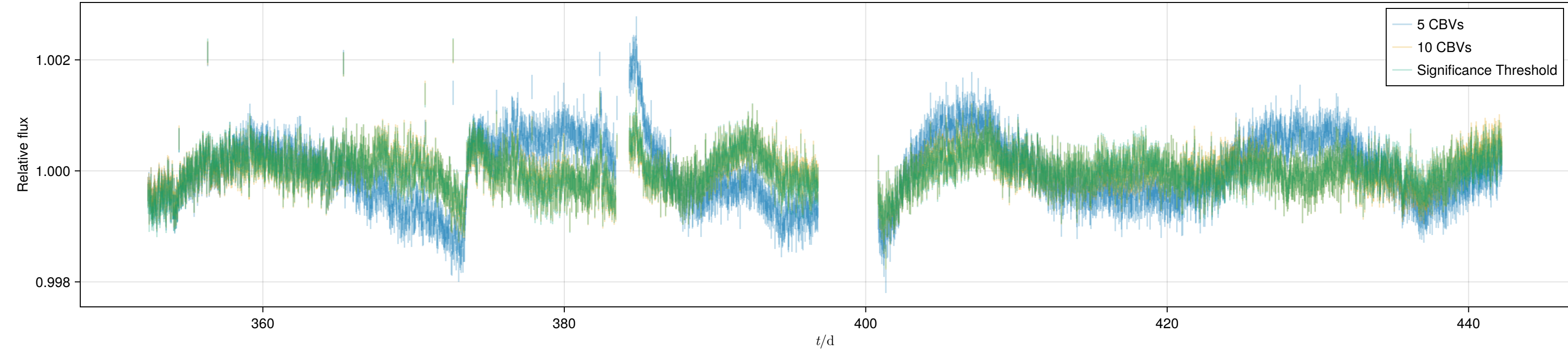
hlsp_iris_kepler_kepler_kplr002570505-q04_kepler_v1.0_lc_detrended.fits
