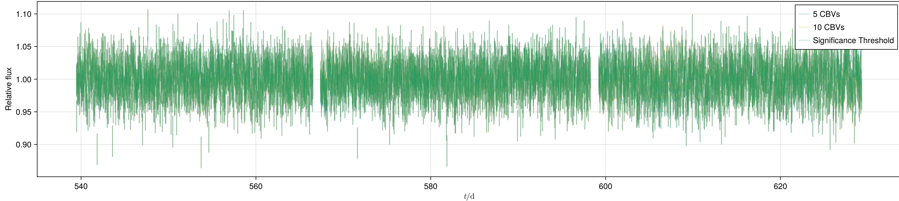
hlsp_iris_kepler_kepler_kplr002707997-q06_kepler_v1.0_lc_detrended.fits
