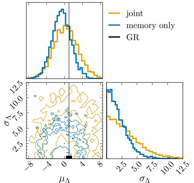
FIG. 2. Mean and standard deviation (see Eq. (3.16)) of the memory enhancement factor across the population of events up to the GWTC-5.0 catalog [54]. Contours represent the 1\sigma , 2\sigma , and 3\sigma credible regions. The yellow contours correspond to simultaneously fitting the memory hyperparameters and the astrophysical population parameters, while the blue contours correspond to fitting only the two memory hyperparameters. The black marker/line represents the GR prediction for the memory distribution: a delta function at 1 - \mu_\Lambda = 1 , \sigma_\Lambda = 0 .
