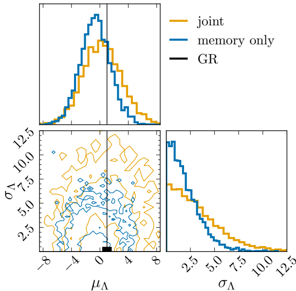
FIG. 2. Mean and standard deviation (see Eq. (3.16)) of the memory enhancement factor across the population of events up to the GWTC-5.0 catalog [53]. Contours represent the 1\sigma , 2\sigma , and 3\sigma credible regions. The yellow contours correspond to simultaneously fitting the memory hyperparameters and the astrophysical population parameters, while the blue contours correspond to fitting only the two memory hyperparameters. The black marker/line represents the GR prediction for the memory distribution: a delta function at 1 - \mu_\Lambda = 1 , \sigma_\Lambda = 0 .
