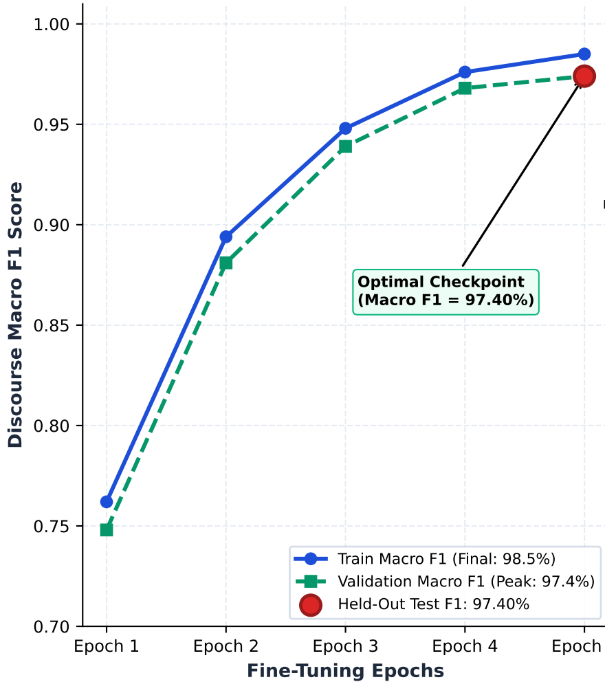
(b) IndoBERT Base Fine-Tuning Convergence
