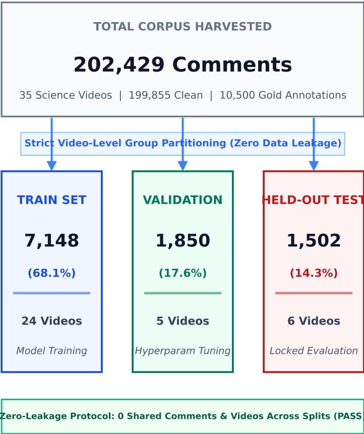
(a) Video-Stratified Zero-Leakage Data Partitioning
