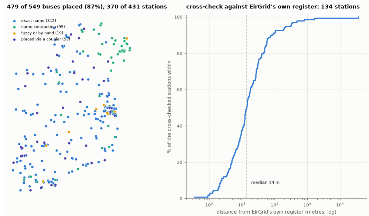
Figure 2: Left: where the WP2024 transmission buses landed, coloured by how each was matched. Right: the cross-check against the station layer of EirGrid's own Transmission Development Plan service. 134 of the matched stations appear in both, at a median separation of 14 metres , which is the difference between one corner of a substation and another. The 95th percentile is 252 metres.
