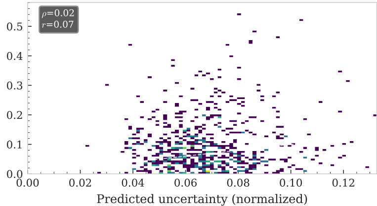
Radial
