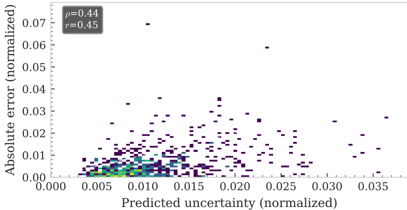
Deep Ens.
