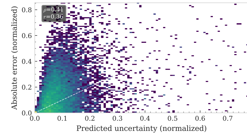
Deep Ens.
