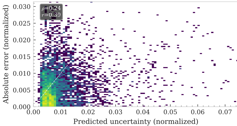
Deep Ens.
