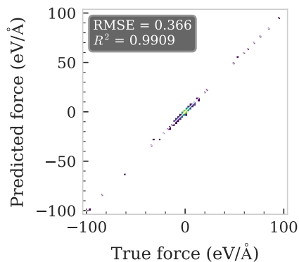
Radial
