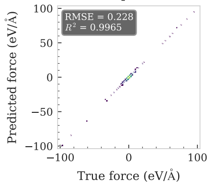
Deep Ens.
