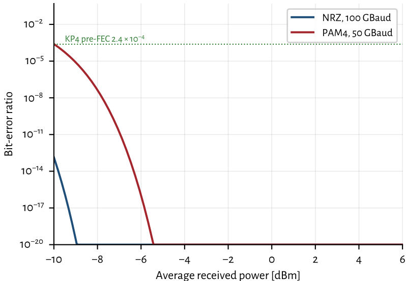
Same 100 Gb/s: PAM4's level penalty vs. NRZ's bandwidth cost
