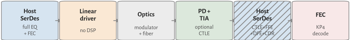
(C) LPO (simplest module; host carries the EQ)
