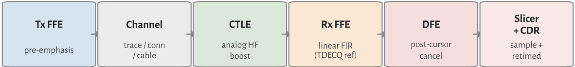
(A) Correct SerDes EQ order (one electrical lane)
