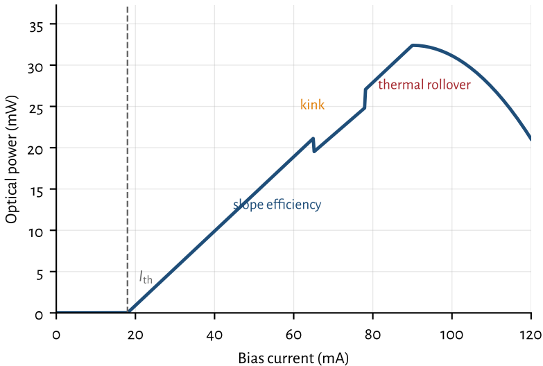
Schematic LIV (not measured data)
