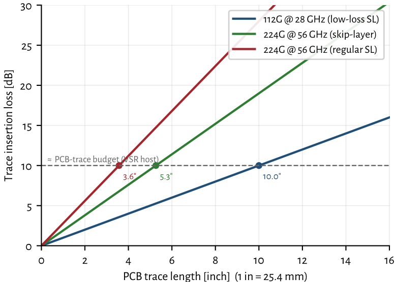
Doubling the baud rate halves the copper reach
