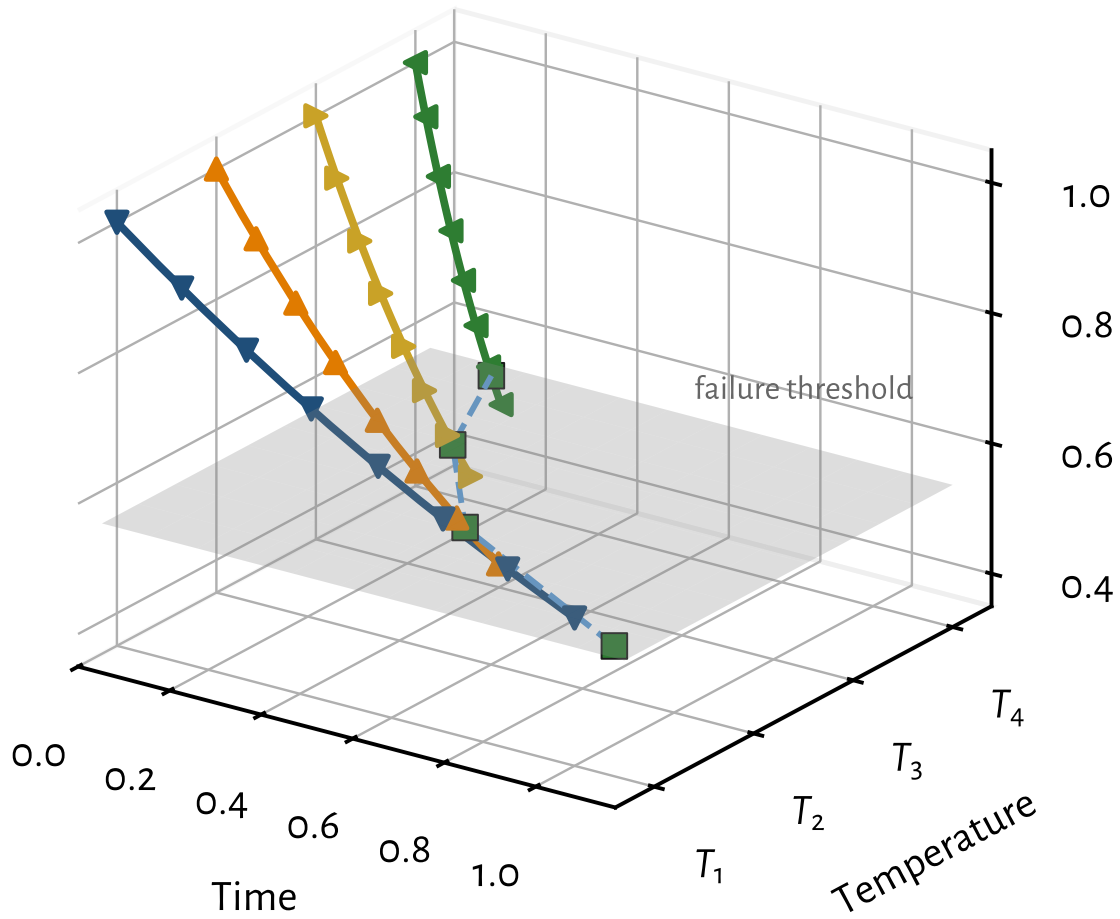
Figure 6.2: Schematic accelerated aging for gradual laser wear-out. A degradation parameter (for example optical power at fixed bias, or threshold current rise mapped to a falling health metric) is tracked versus time at several stress temperatures T_1 < T_2 < T_3 < T_4 . Higher temperature reaches the failure threshold sooner. The dashed curve on the threshold plane is the time-to-failure trend that Arrhenius acceleration turns into a use-condition life estimate. Not measured data. Valid only for one thermally activated mechanism with junction temperature as the stress variable; sudden modes such as COD or ESD do not draw this surface.
