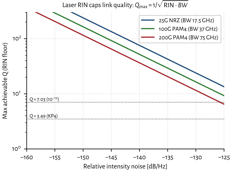
Figure 5.3: The RIN ceiling Q_{\max} = 1/\sqrt{\text{RIN} \cdot \text{BW}} . Wider receiver bandwidth (higher lane rate) integrates more RIN, lowering the ceiling. Where a curve dips below the dotted anchors, that link can no longer reach the corresponding BER.
