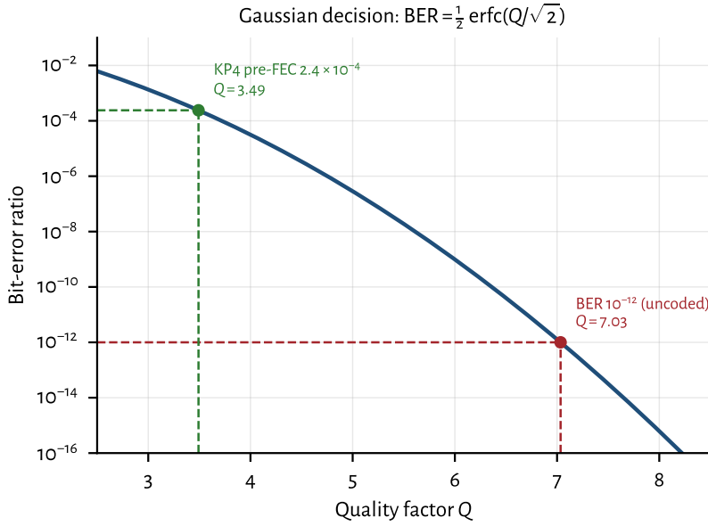
Figure 5.1: The Gaussian decision curve. Every dB of Q buys orders of magnitude of BER near the knee, which is why FEC (trading a modest Q for a huge BER improvement) is decisive.
