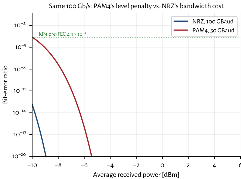
Figure 5.5: NRZ (100 GBaud) versus PAM4 (50 GBaud) at the same 100 Gb/s. PAM4 pays a level penalty but relaxes bandwidth; the crossover with the KP4 pre-FEC threshold sets the required operating power.
