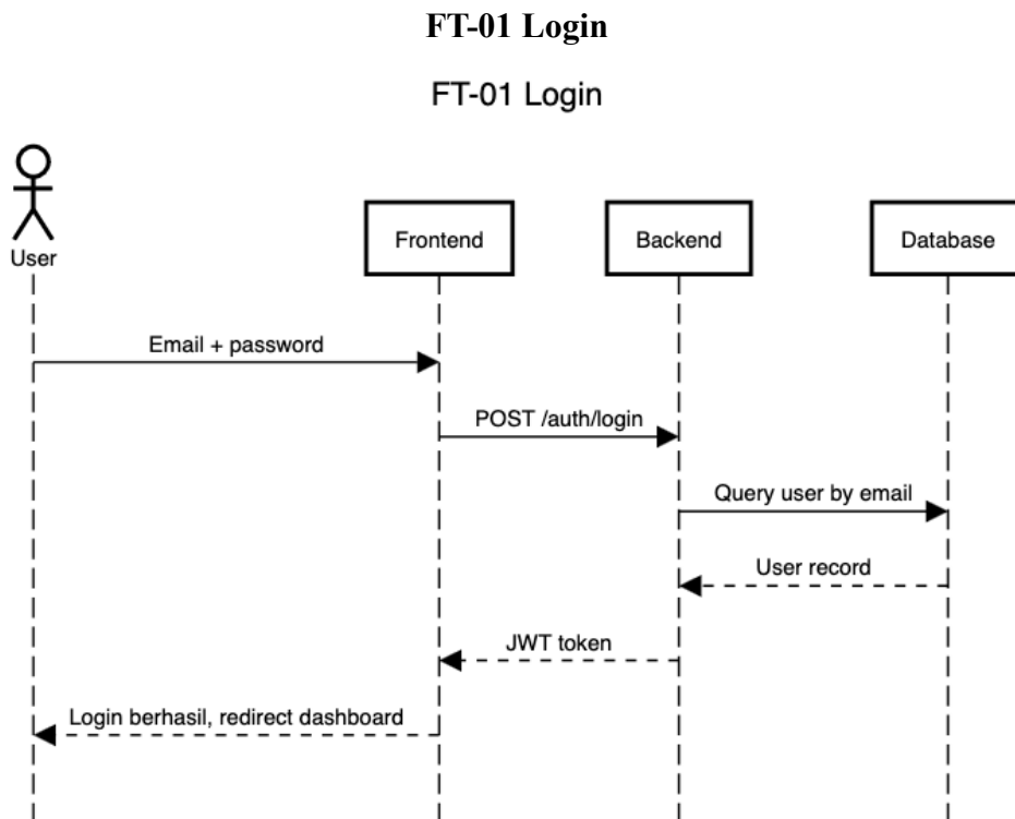
Gambar IV.2 Sequence Diagram FT-01 Login
