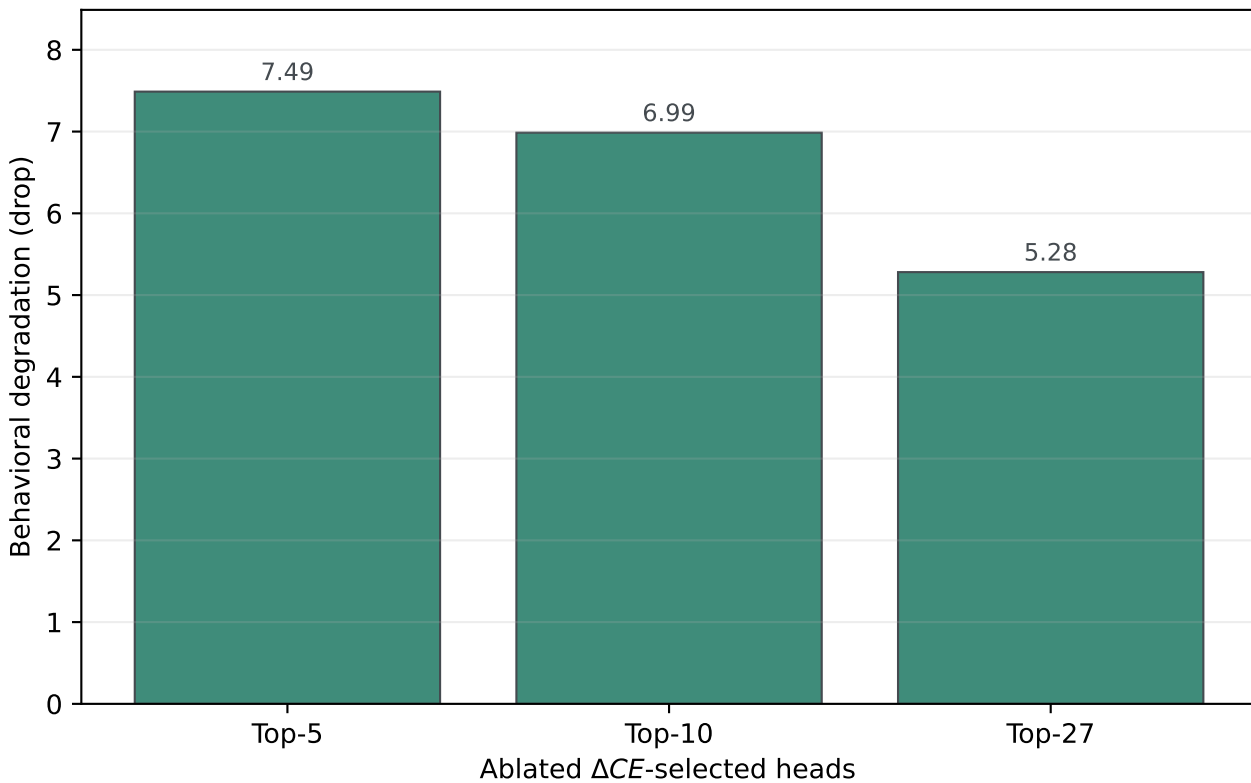
Top- k causal ablation of selected attention heads
