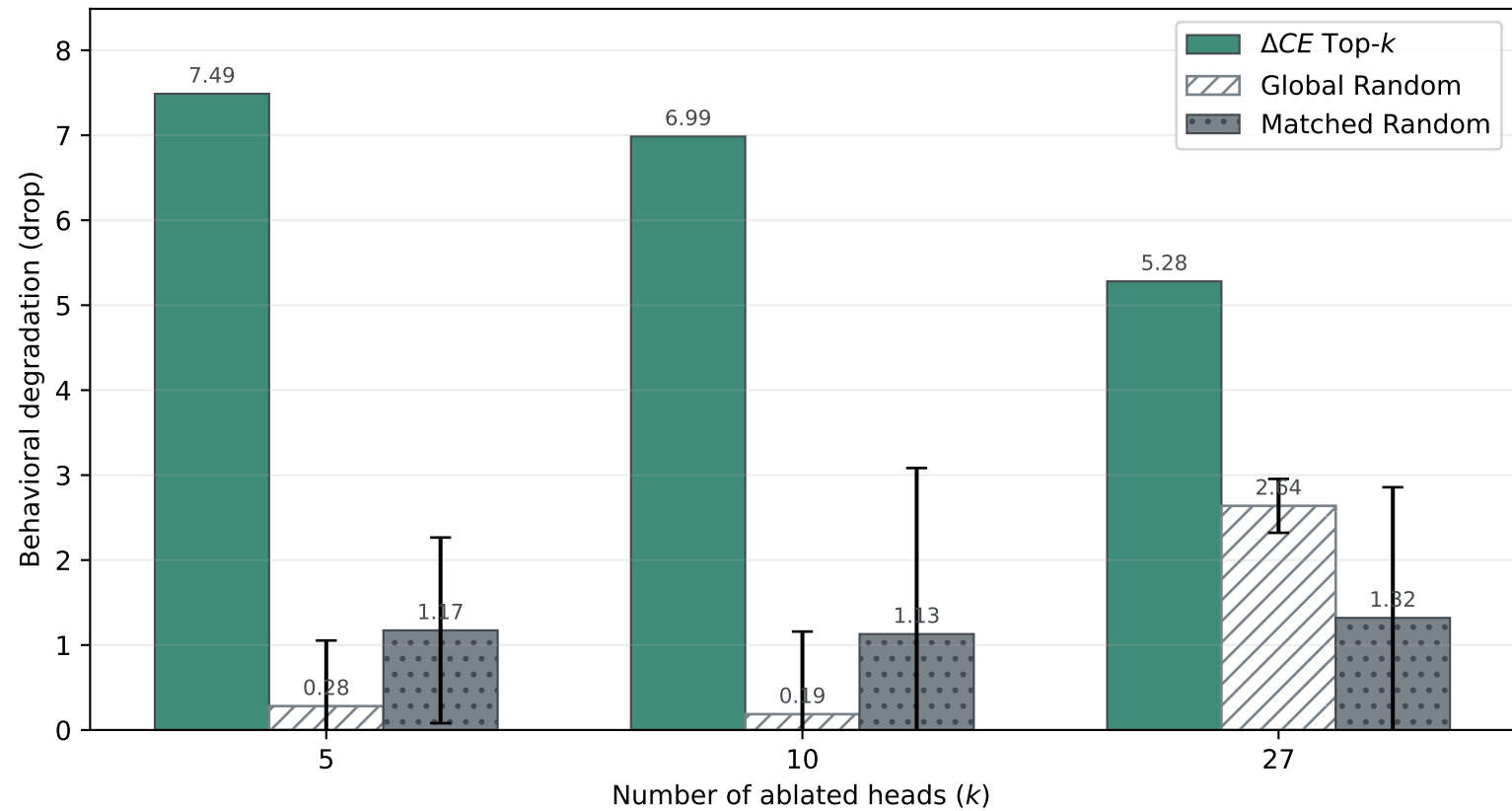
Top-k ablation compared with random controls
