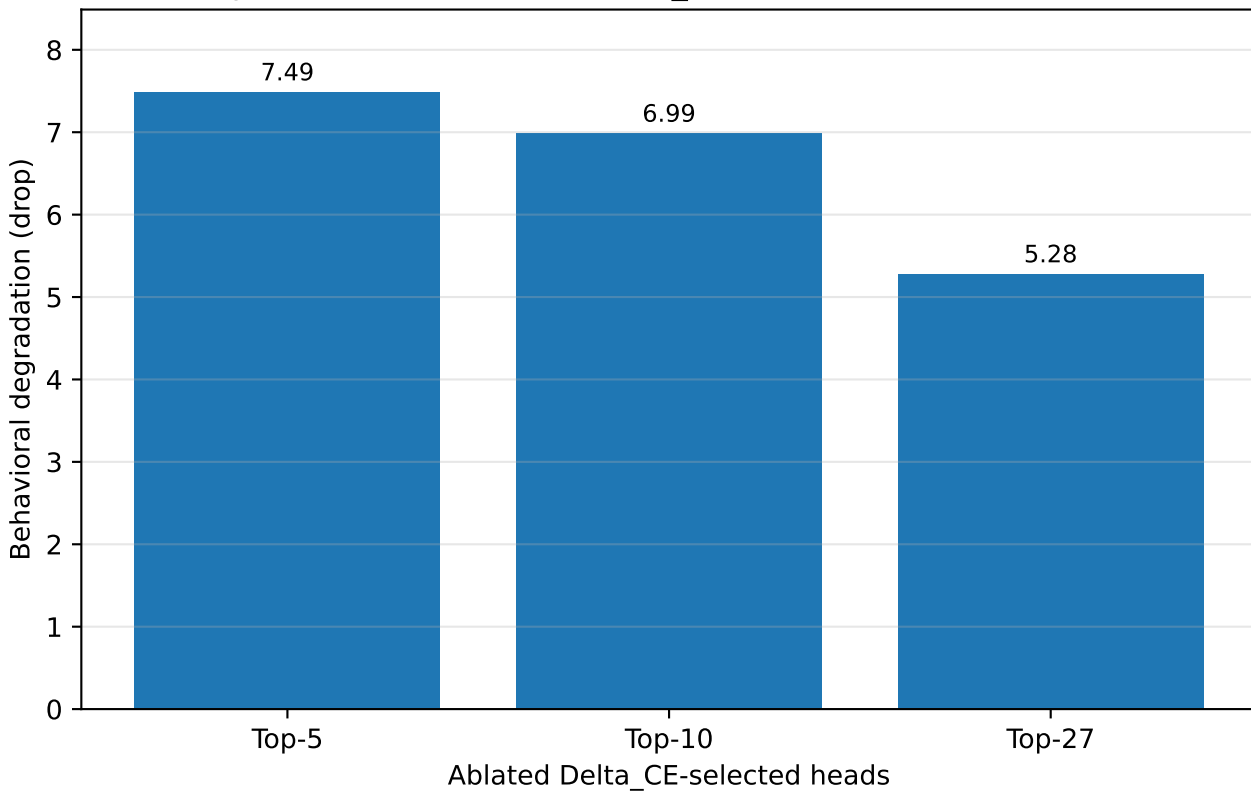
Top-k causal ablation of Delta_CE-selected attention heads
