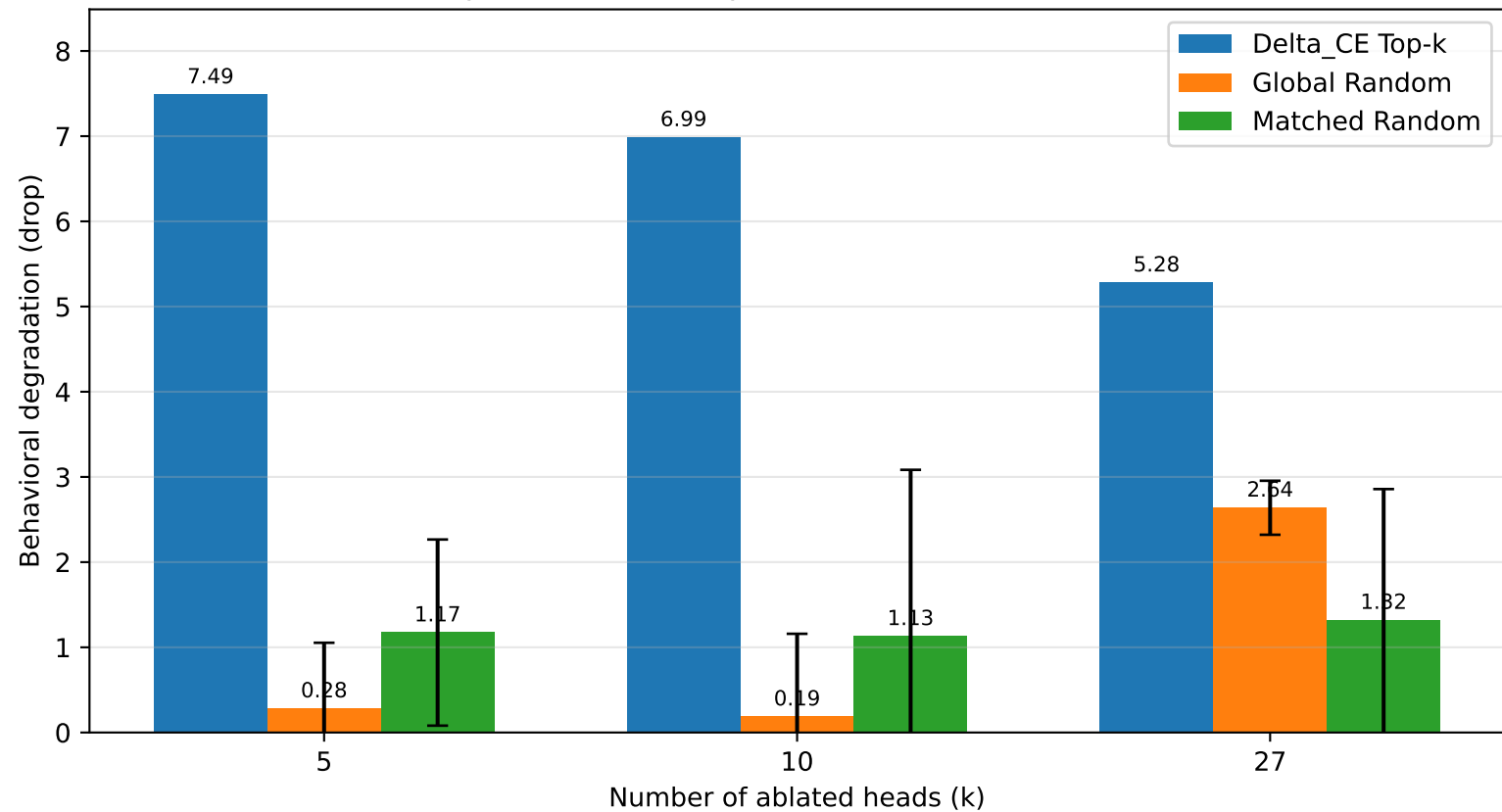
Top-k ablation compared with random controls
