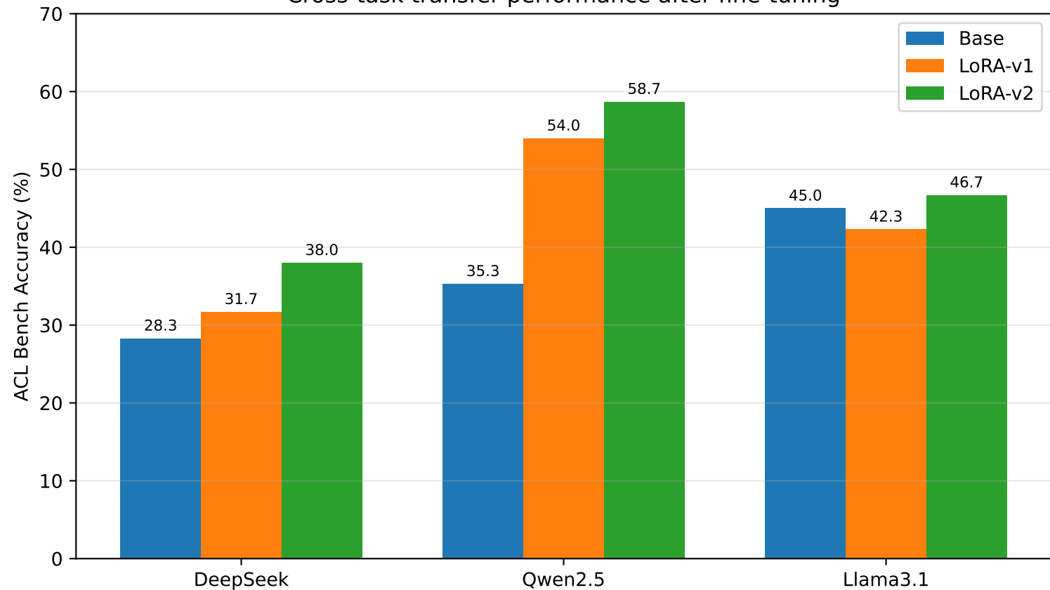
Cross-task transfer performance after fine-tuning
