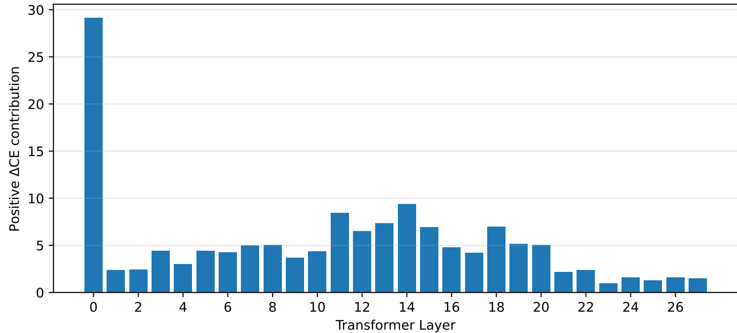
Layer-wise distribution of causal contribution
