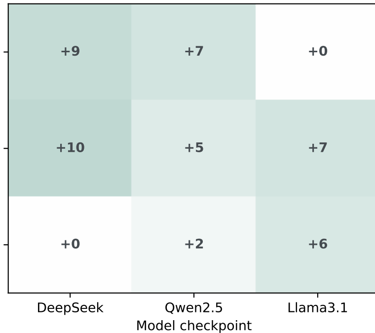
DD-LoRA → RC-LoRA
