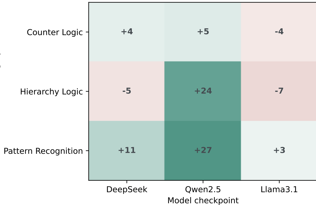
Base → DD-LoRA
