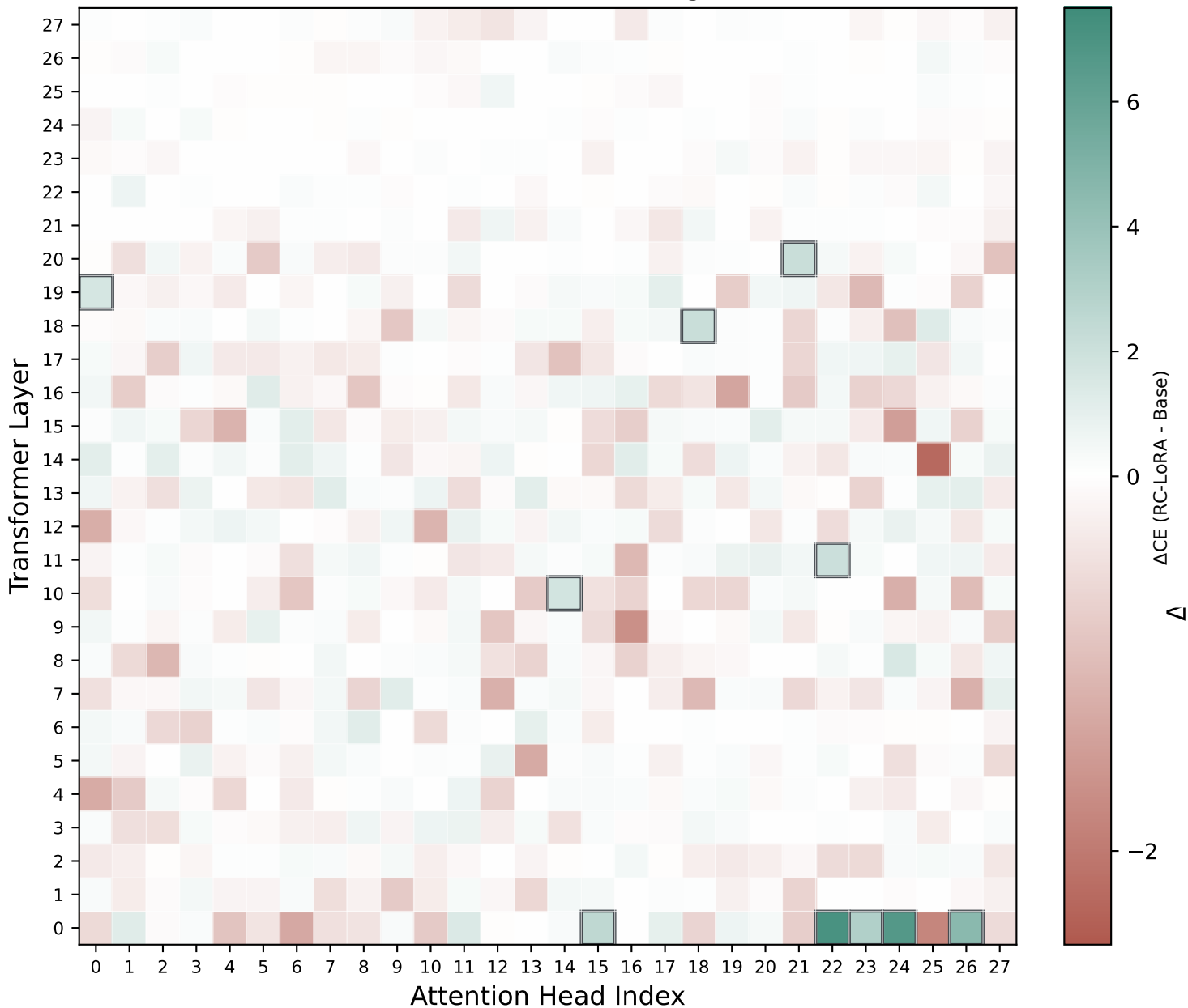
Attention-Head Causal Change ( \Delta CE )
