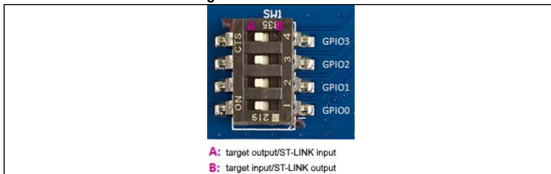
Figure 18. B-STLINK-VOLT
