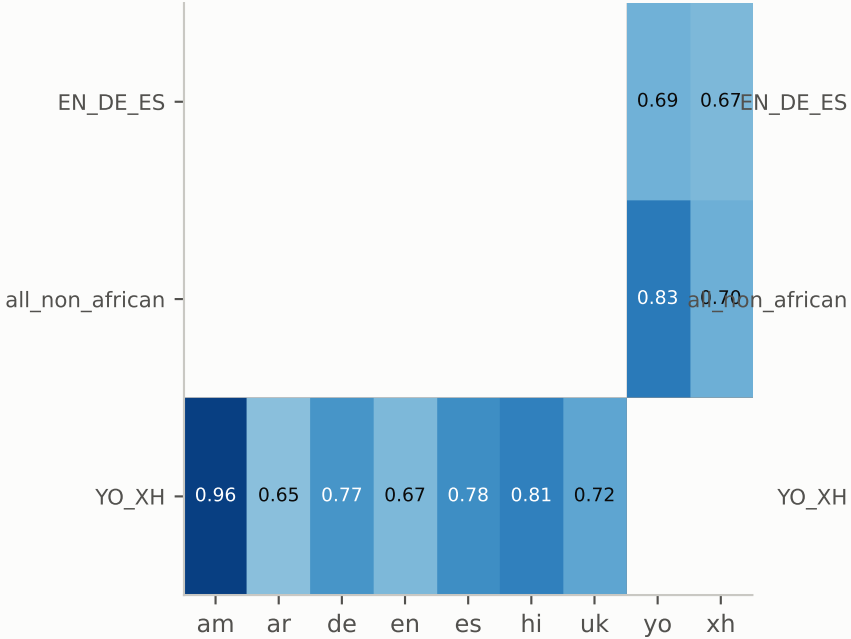
Fig 2 — Probe transfer matrix [ASSOCIATIVE evidence: no causal test]
