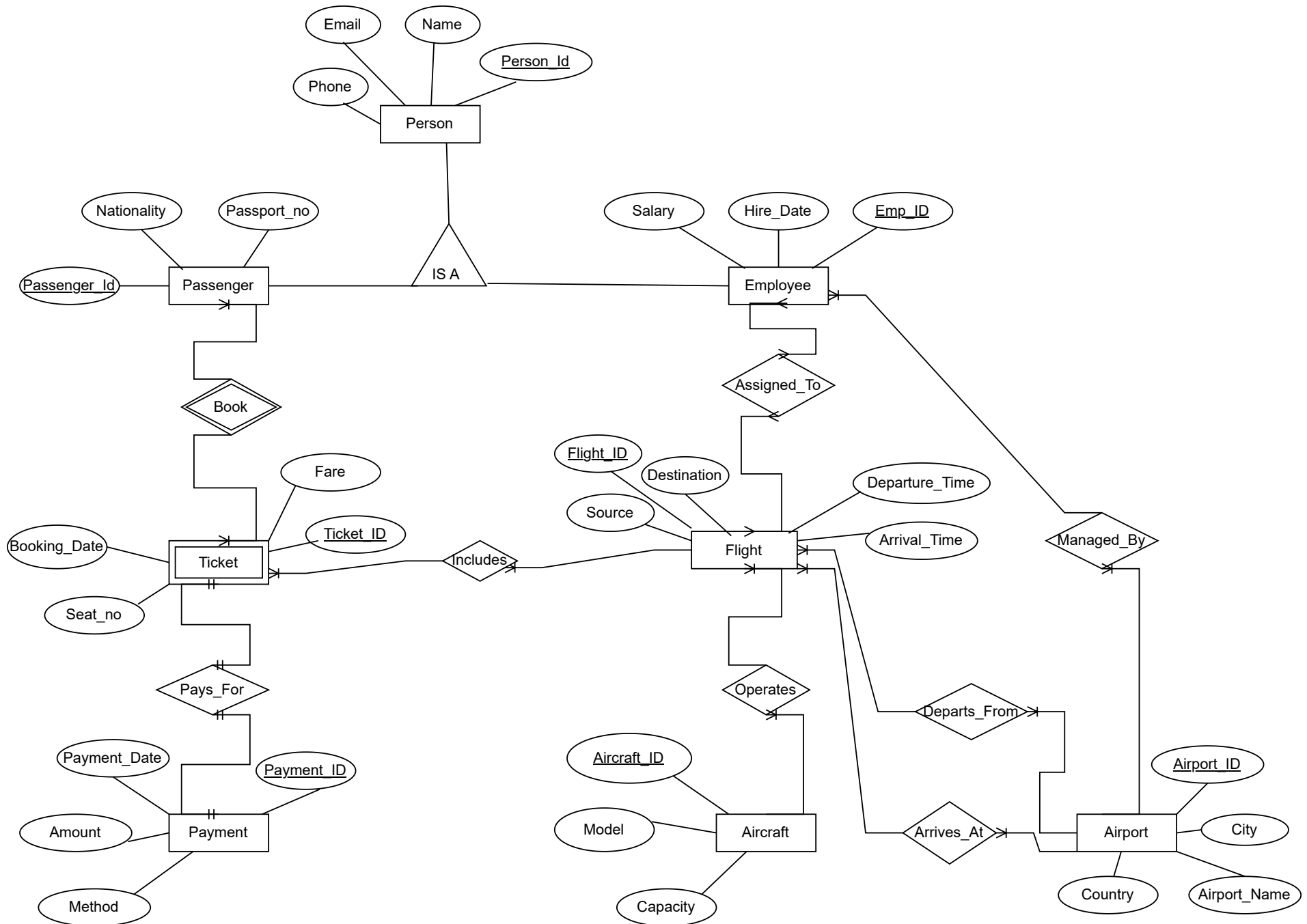
“Enhanced Entity Relationship Diagram (EERD) — Airline Reservation System”.
