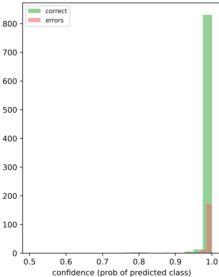
Confidence distribution
