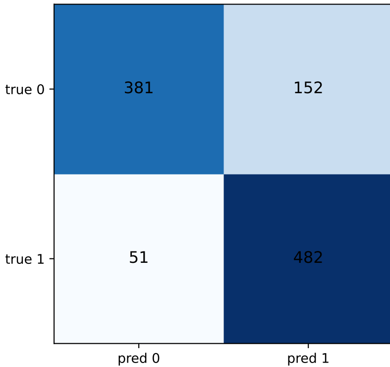
Confusion matrix
