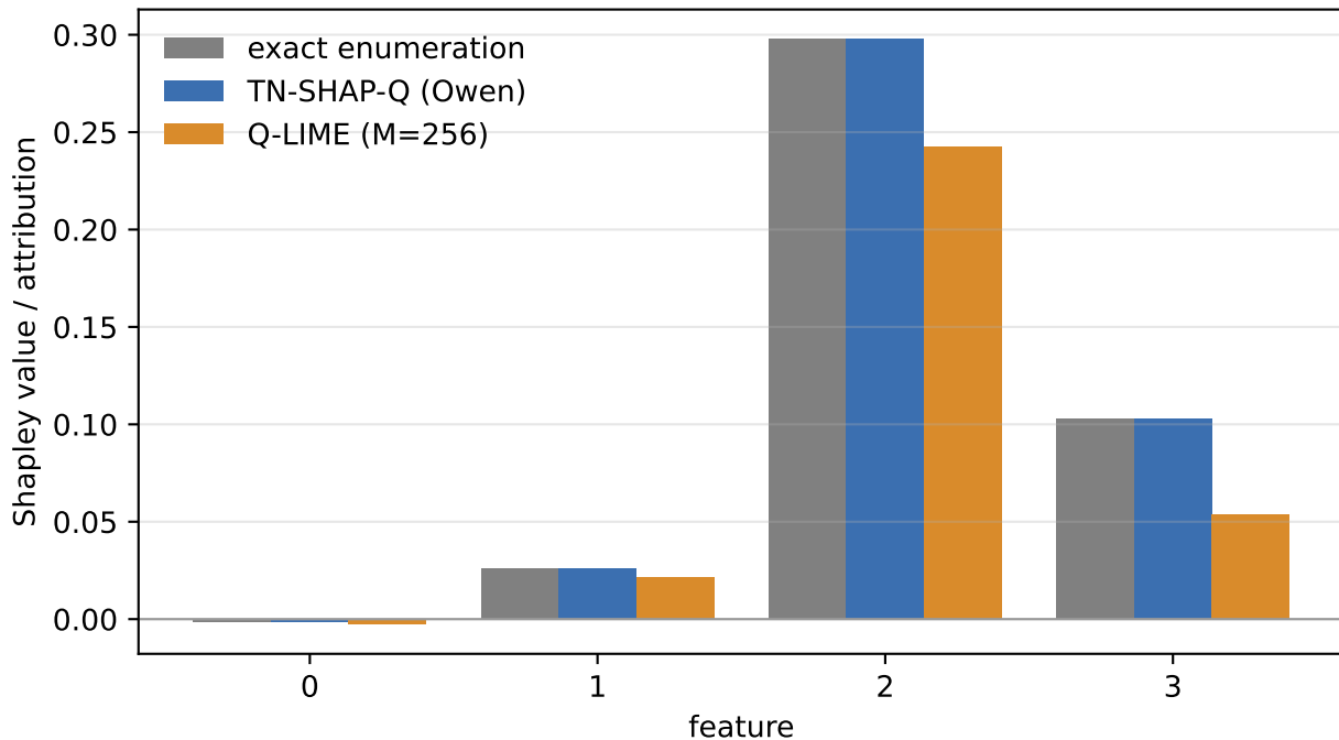
Feature importance: exact vs TN-SHAP-Q vs Q-LIME
