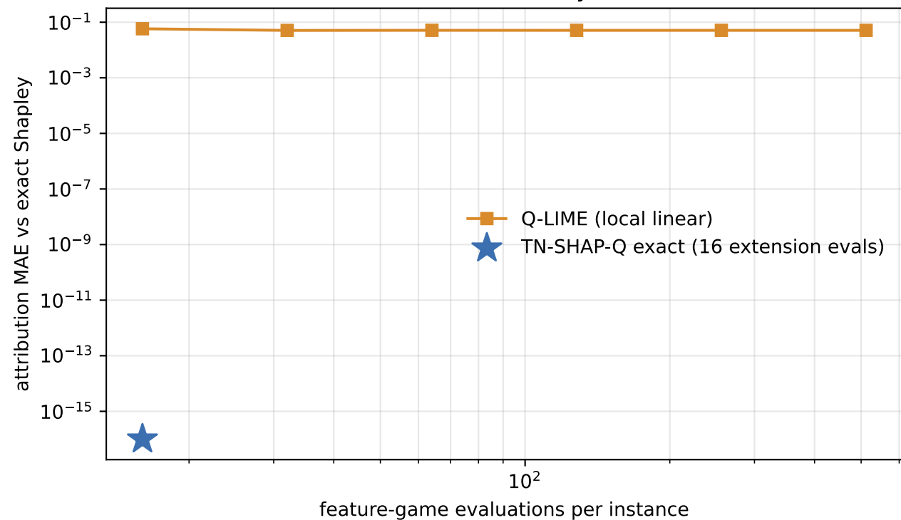
Feature attribution: accuracy vs cost (d=4)
