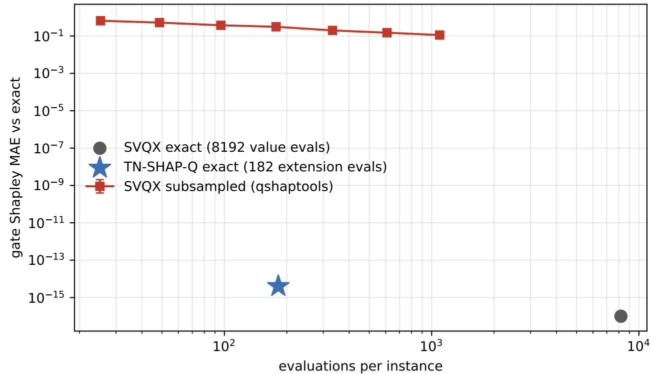
Gate Shapley: TN-SHAP-Q vs SVQX (QAOA, m=13)
