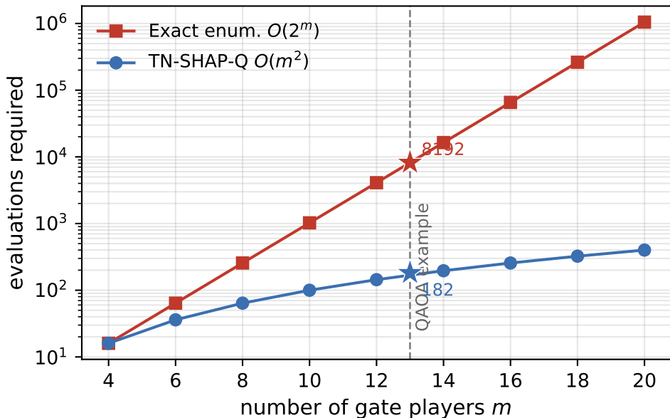
Exact gate Shapley: cost vs circuit size
