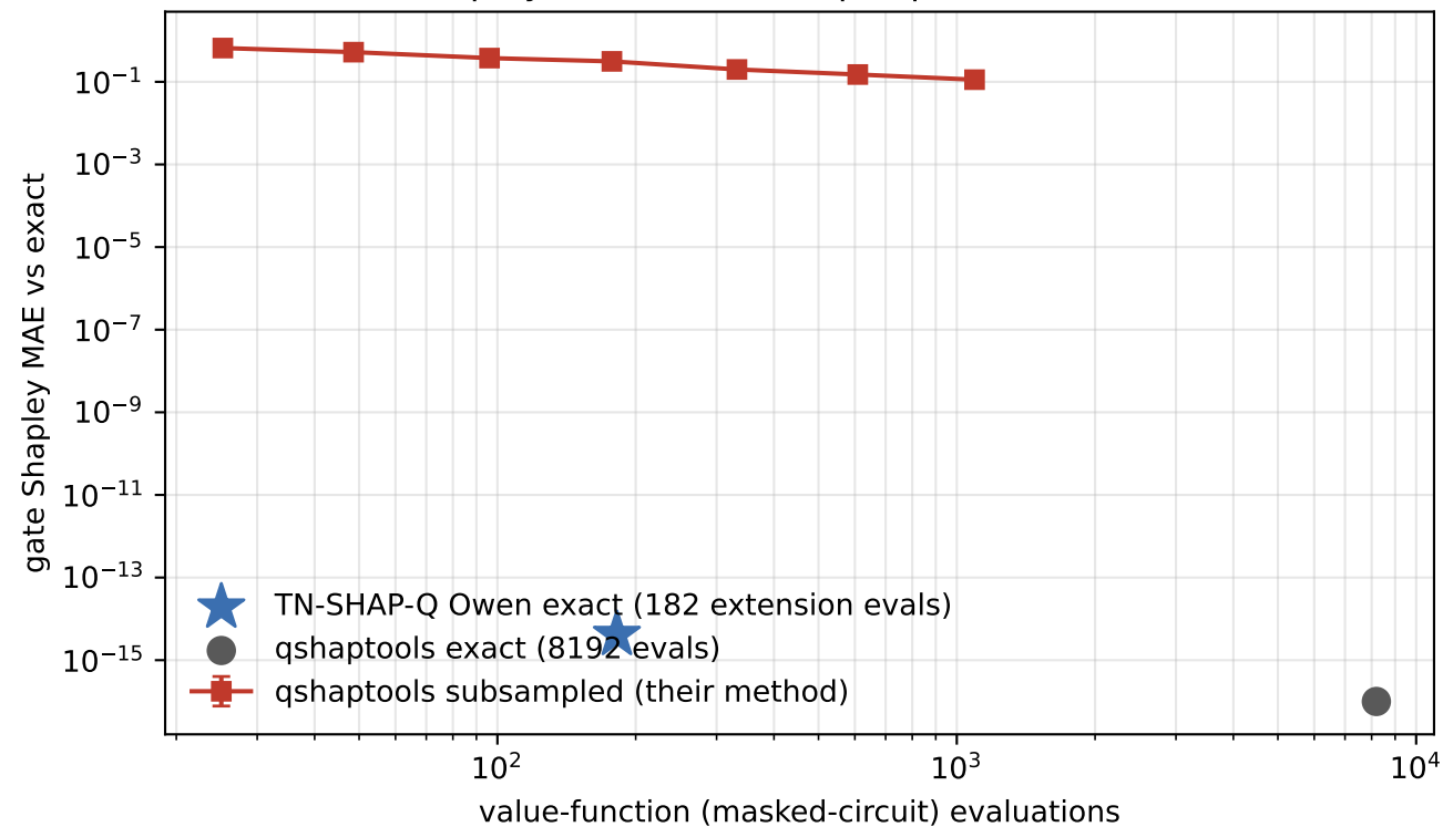
Gate Shapley: TN-SHAP-Q vs qshaptools (QAOA, m=13)
