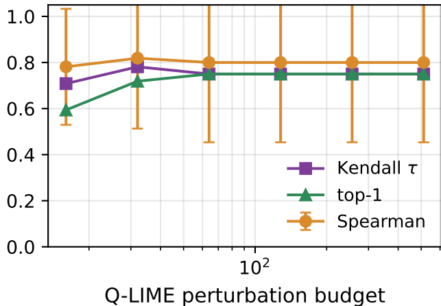
(b) Q-LIME ranking (saturates < 1 )
