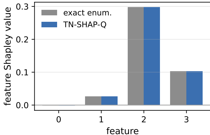
(a) Exact vs TN-SHAP-Q (MAE 5 \times 10^{-17} )
