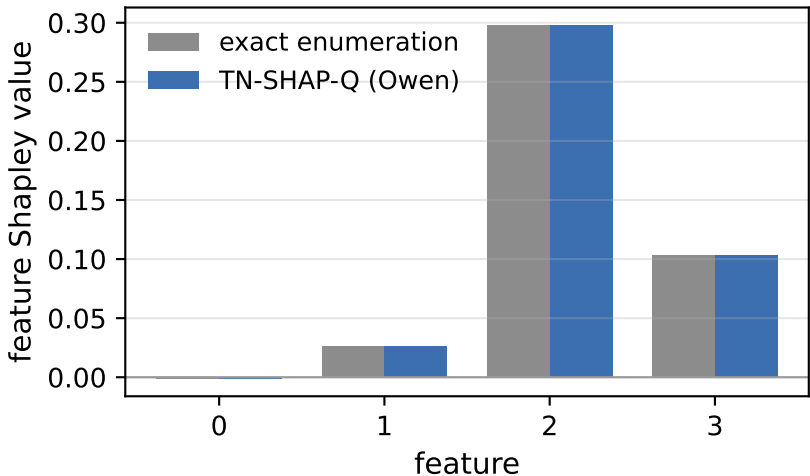
Exact vs TN-SHAP-Q (coincide)
