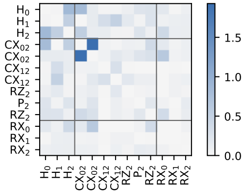
(a) |I(\{i,j\})| by gate (layer-ordered)
