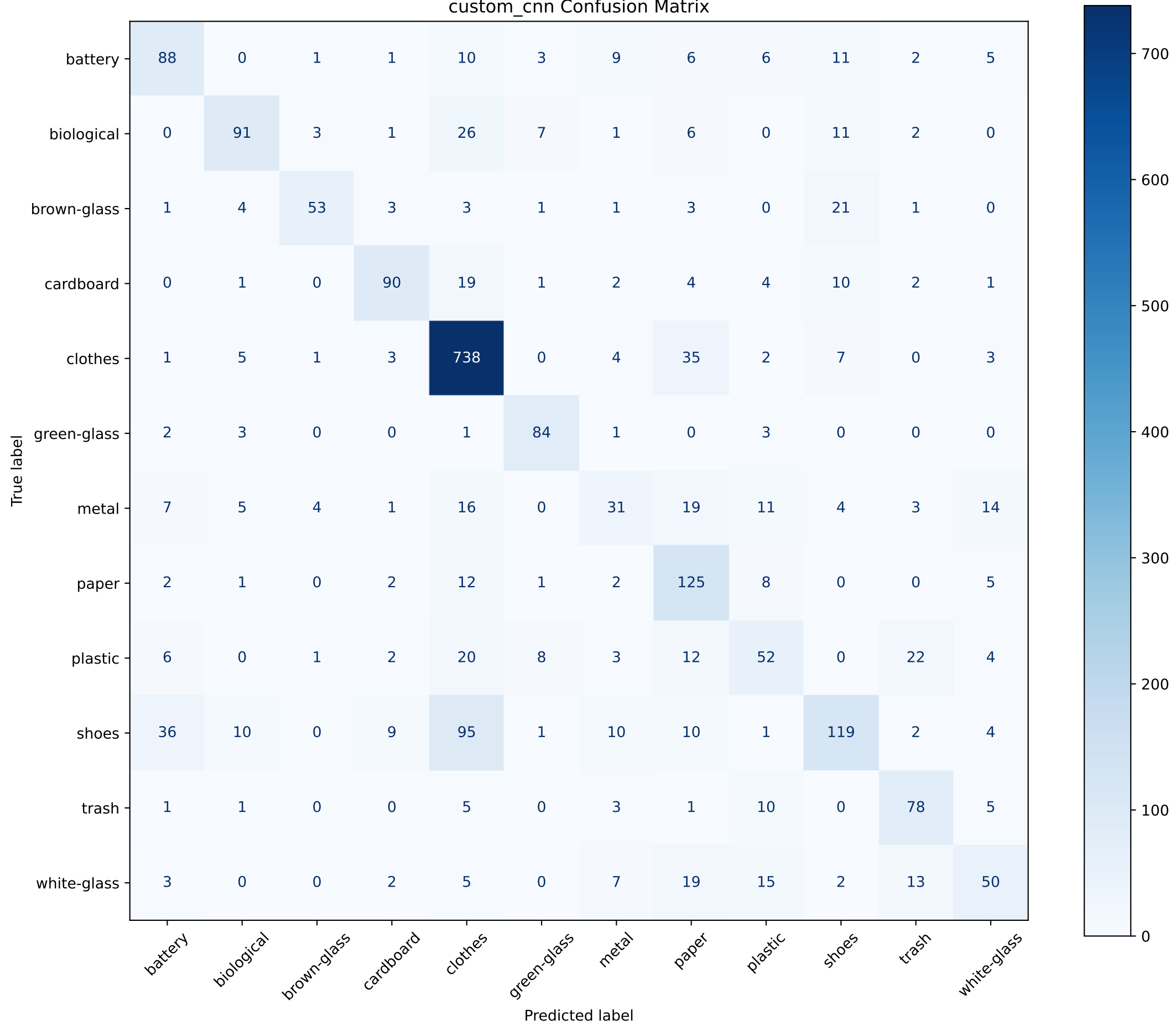
custom_cnn Confusion Matrix
