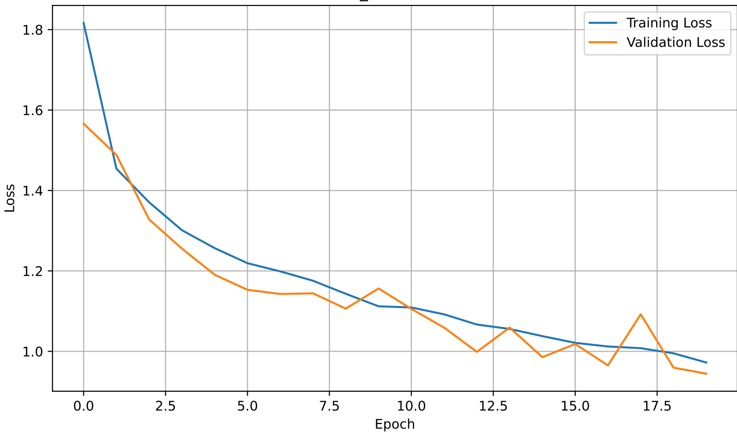
custom_cnn Loss Curve
