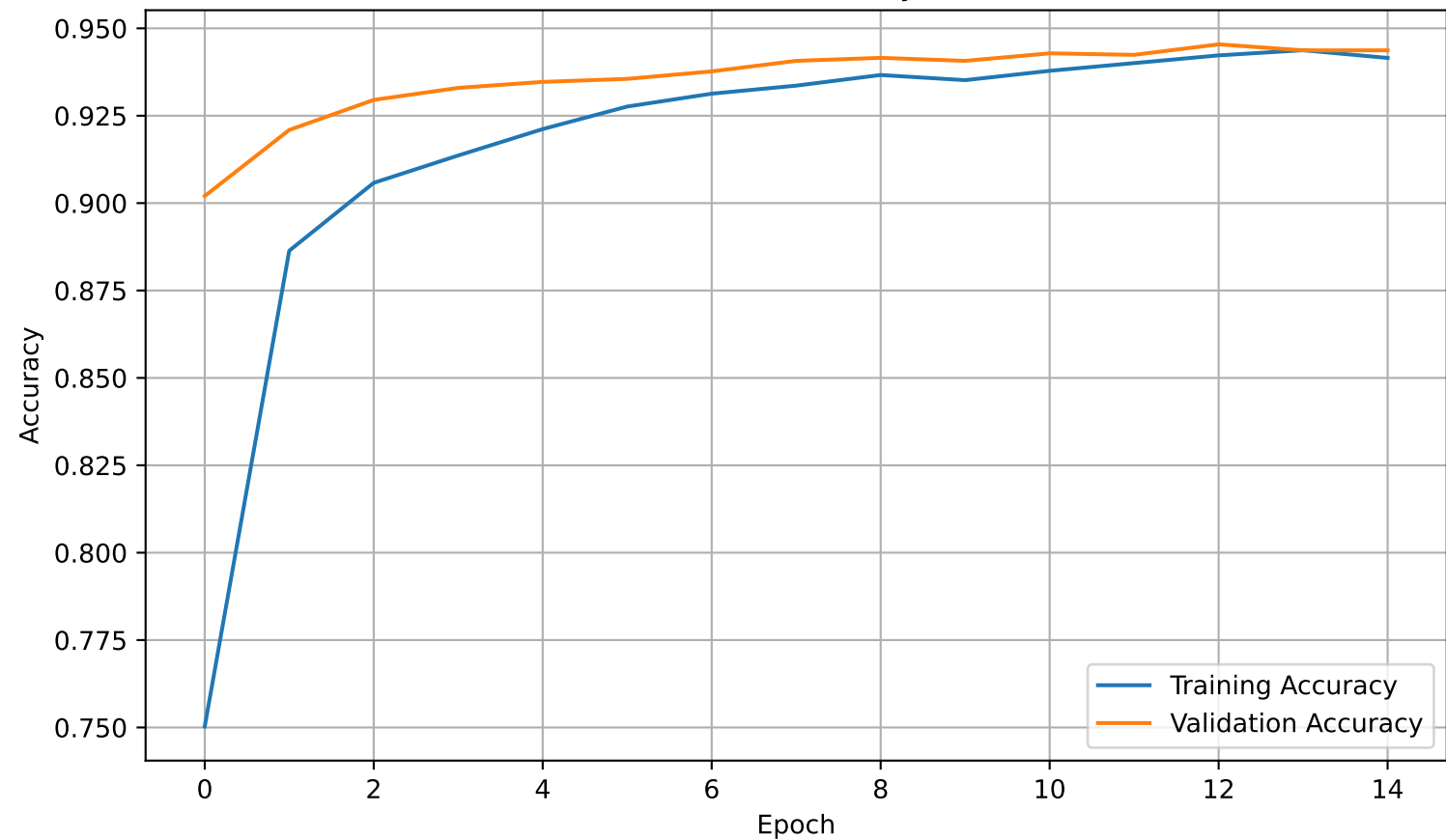
mobilenetv2 Accuracy Curve
