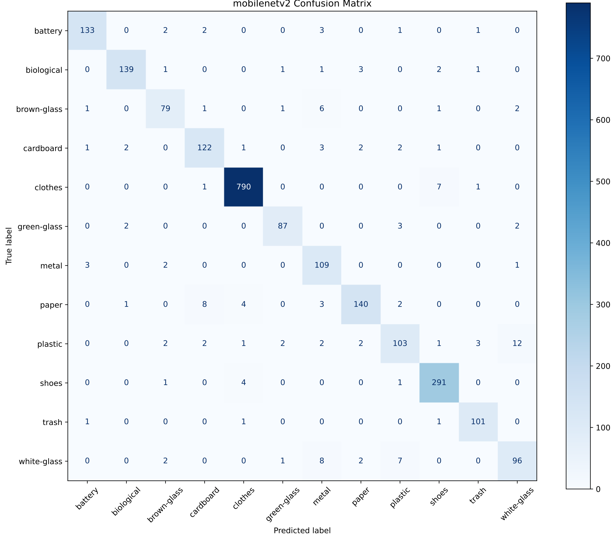
mobilenetv2 Confusion Matrix
