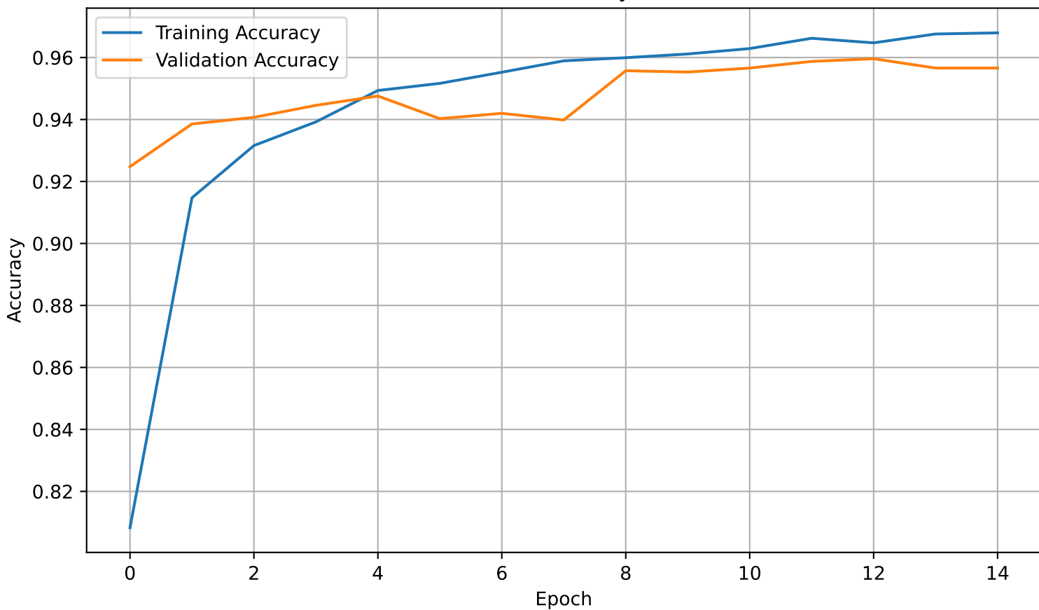
resnet50 Accuracy Curve
