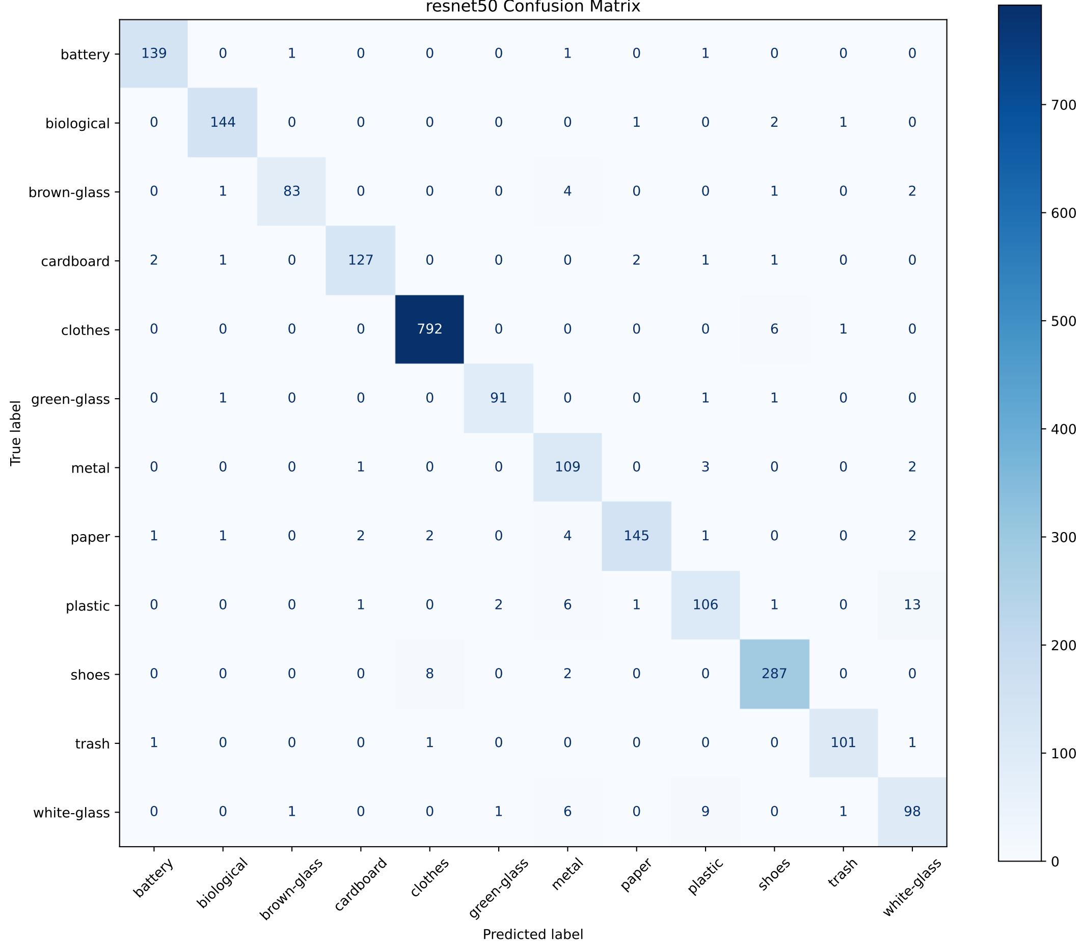
resnet50 Confusion Matrix
