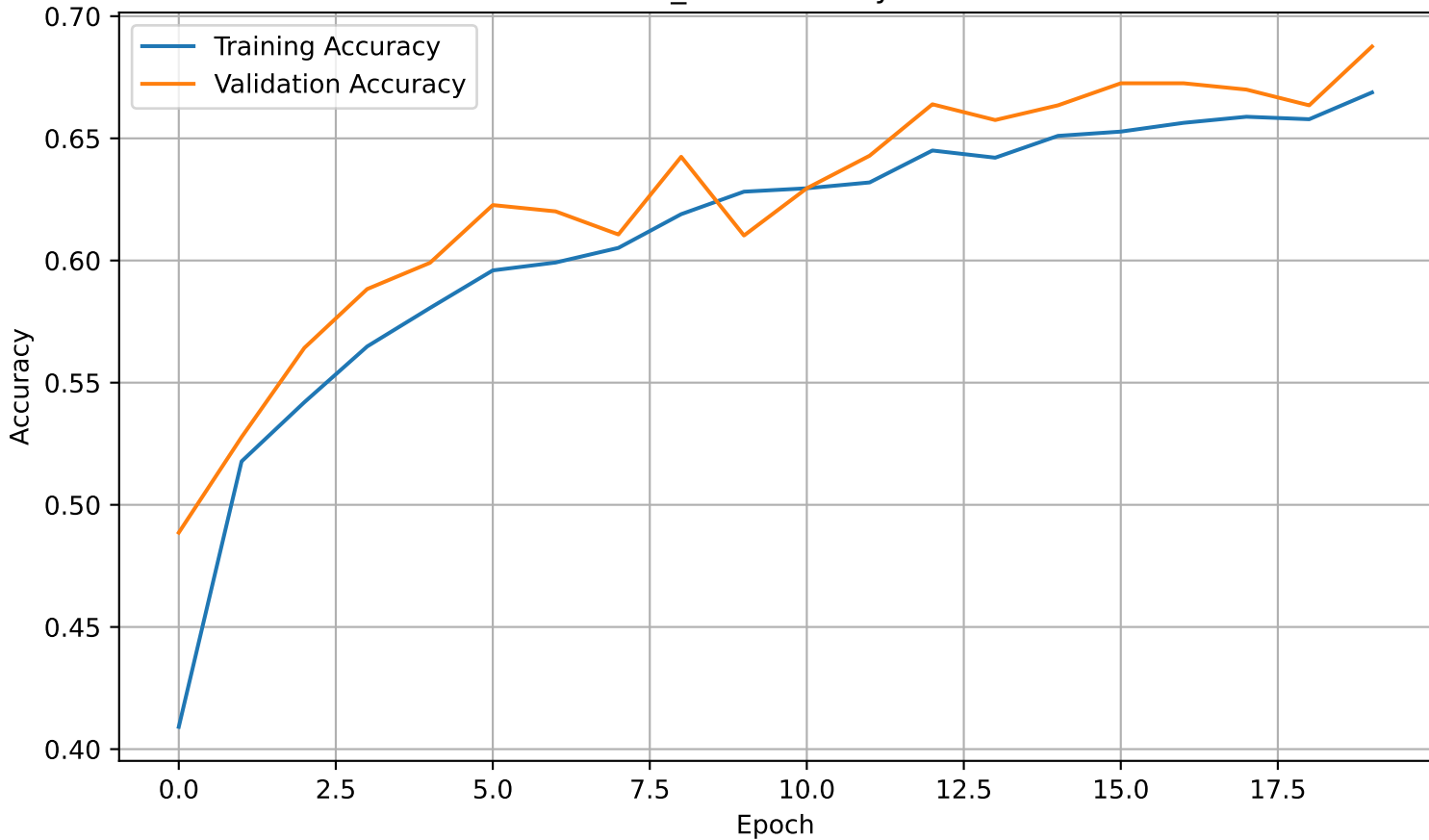
custom_cnn Accuracy Curve
