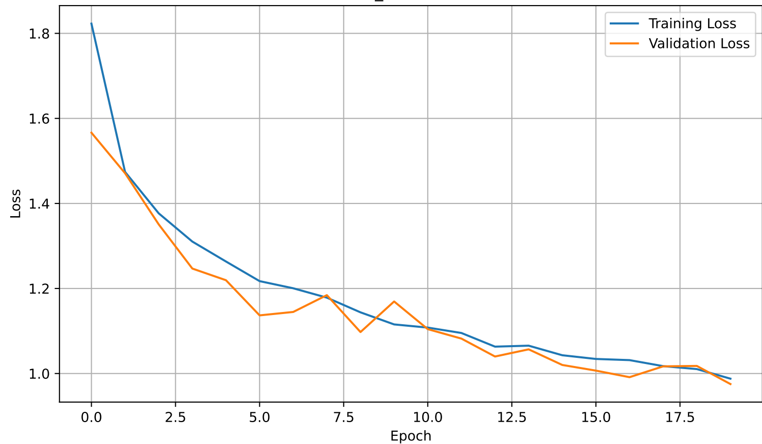
custom_cnn Loss Curve
