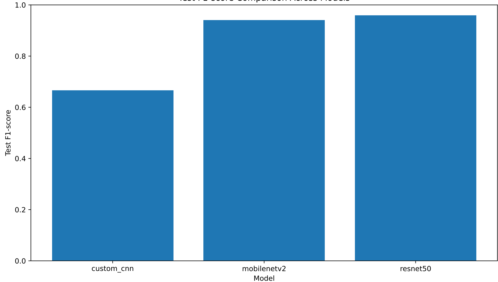
Test F1-score Comparison Across Models
