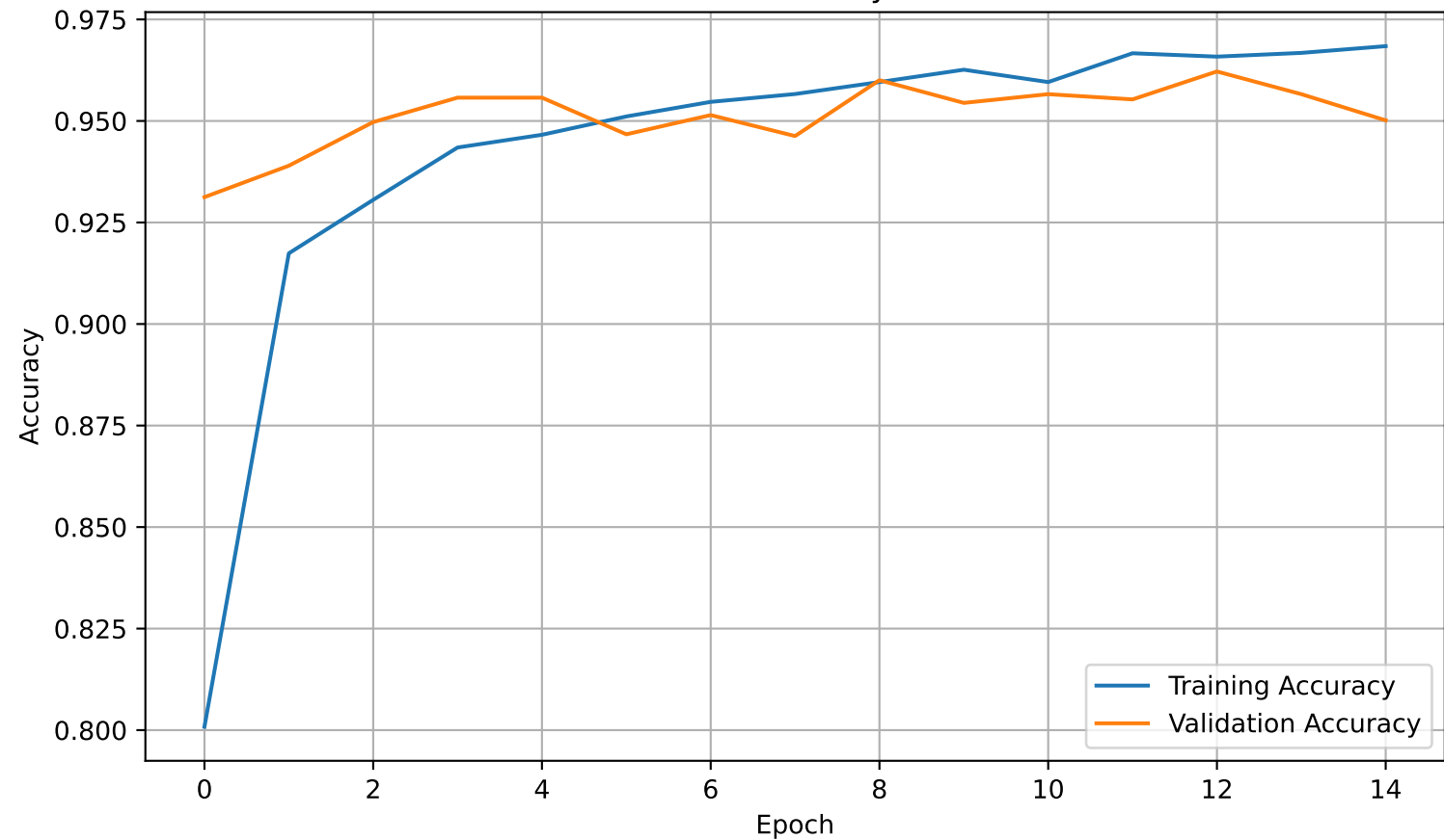
resnet50 Accuracy Curve
